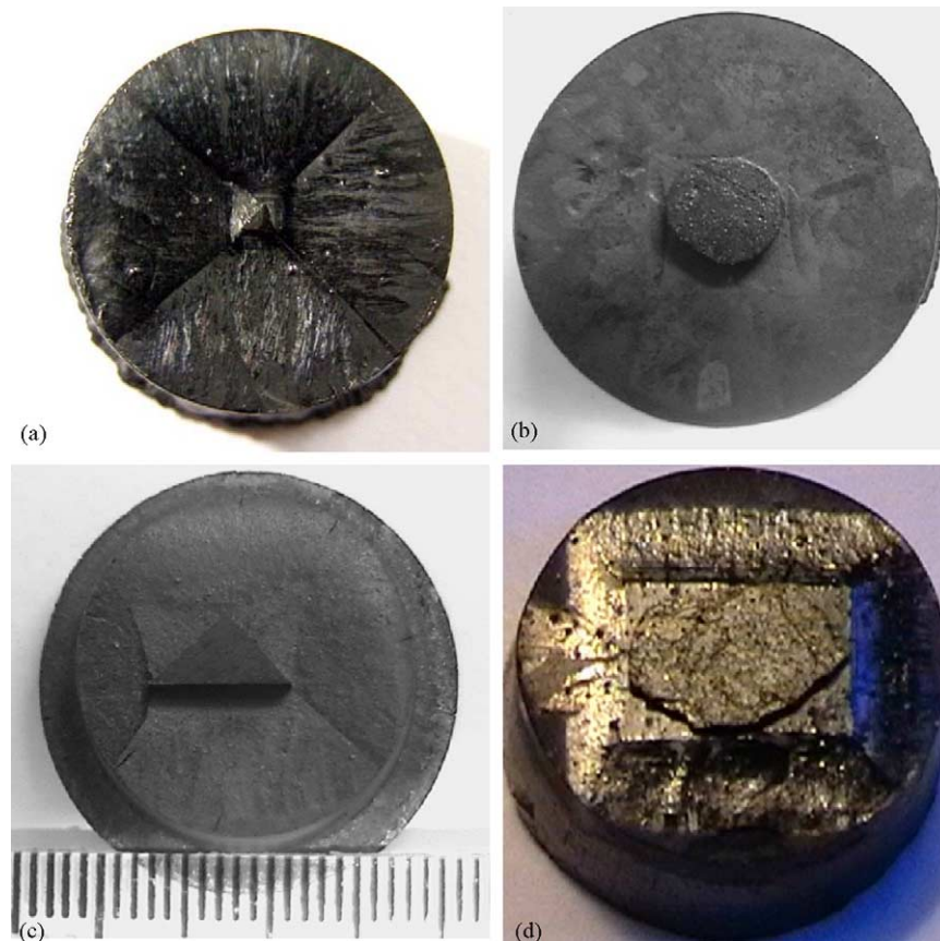
Fig. 1. YBCO samples showing the nucleation and growth of a grain from seed crystals of different morphologies. Initial growth patterns from c -axis oriented seed crystals of (a) square, (b) circular, (c) triangular and (d) irregular seed geometries.
