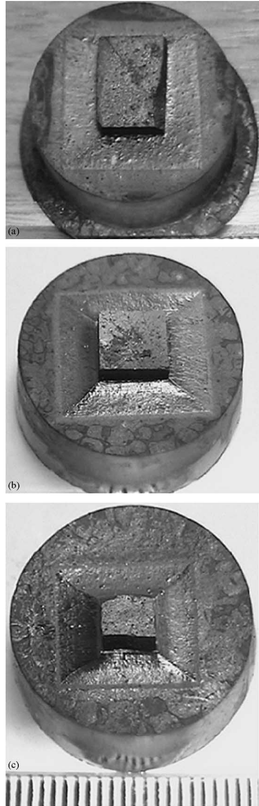
Fig. 3. YBCO grains grown using different size seed crystals under otherwise identical thermal conditions. Increasing the size of the seed crystals results in increasing the size grains within the same processing times.
