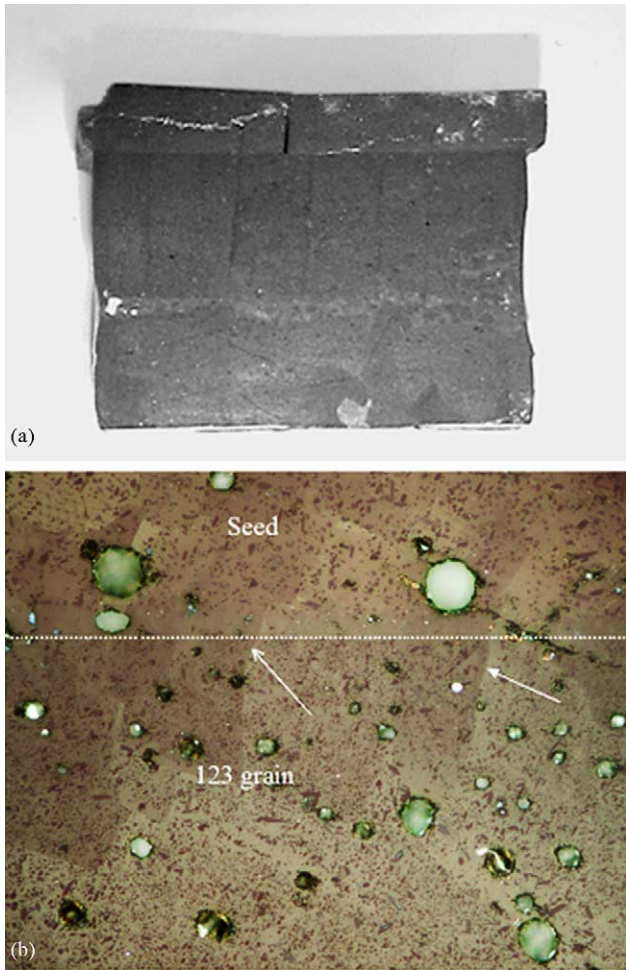
Fig. 2. (a) Cross-section of a YBCO single grain grown using a seed crystal of size larger than that of the preform. (b) The orientation of sub-grains, marked by arrows, from the seed crystals are observed to replicate that of the seed throughout the entire grain.
